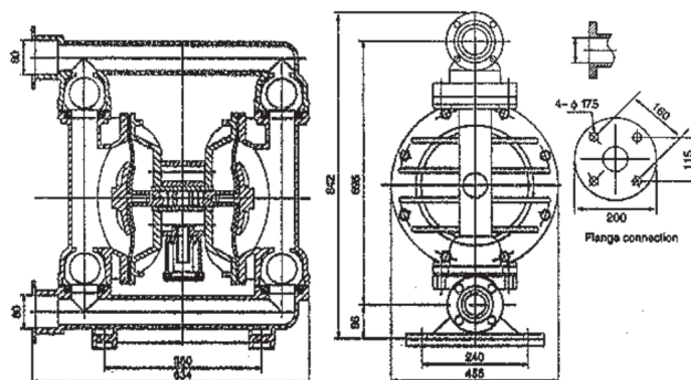
Installation Dimension
