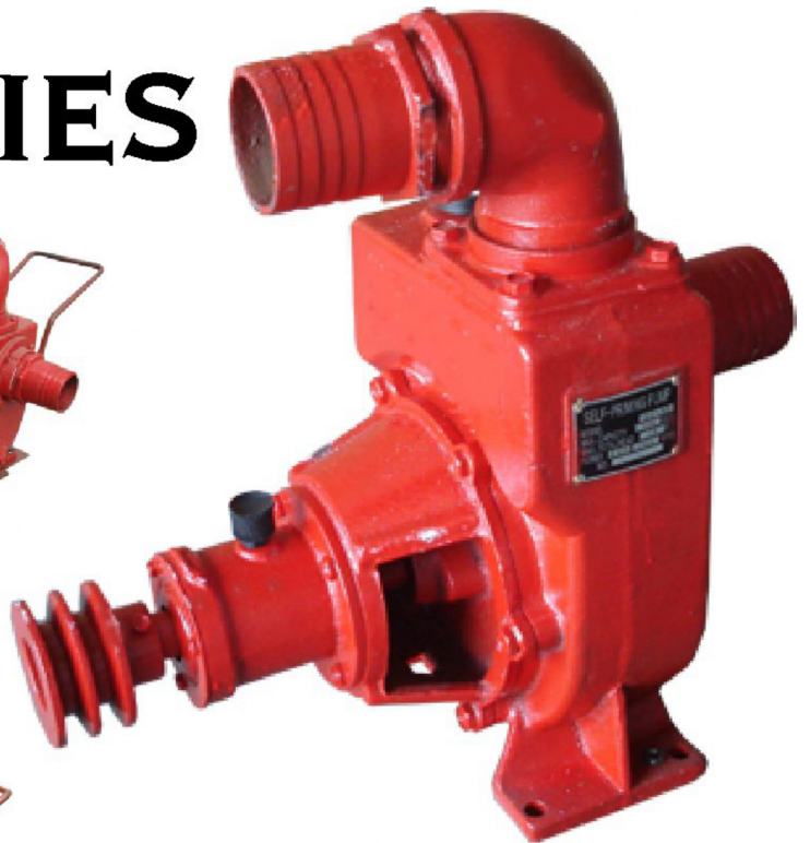
Self Priming Pump NS100 c/w Diesel Engine S195N
